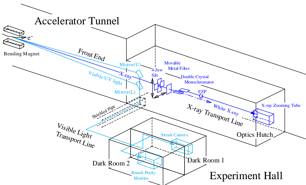
Fig.1 Layout of the accelerator diagnostics beamline I. Components of the beam diagnostics systems are shown.
