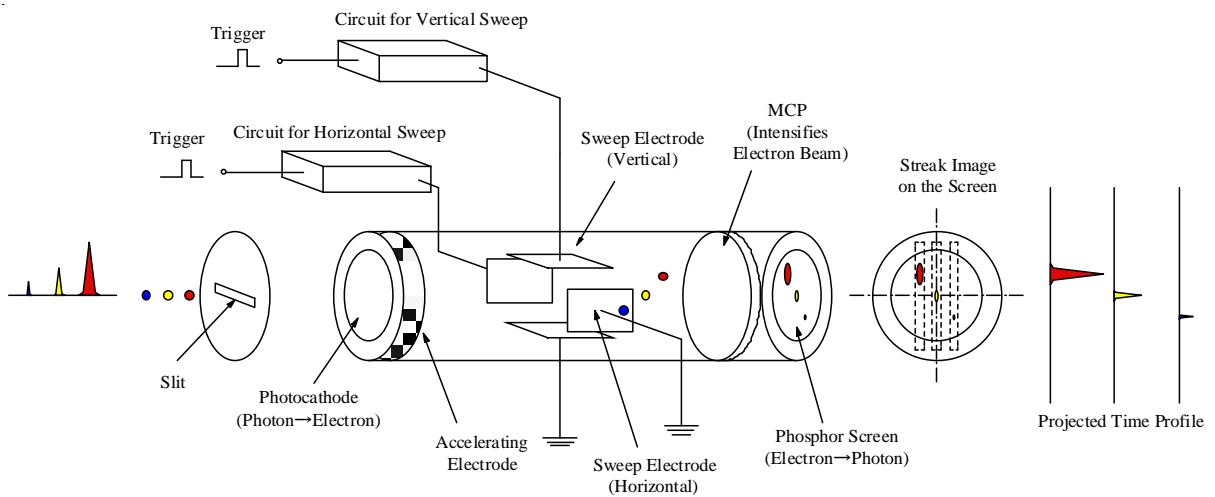
Fig.5 Principle of operation of a streak camera (dual sweep mode).
