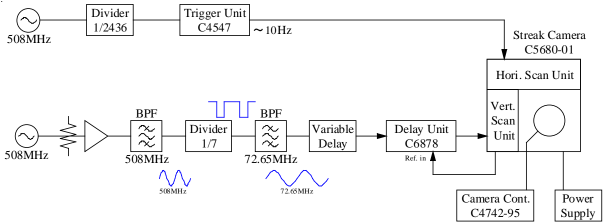
Fig.6 Timing signal system for operating the streak camera.
