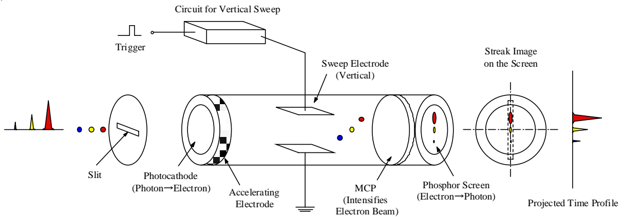
Fig.4 Principle of operation of a streak camera (single sweep mode).
